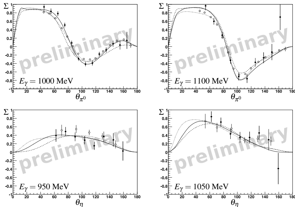
FIGURE 5. Beam asymmetry \Sigma : top: \gamma p \rightarrow p\pi^0 , bottom: \gamma p \rightarrow p\eta . The preliminary data (filled circles) is compared to the GRAAL data[6] for \pi^0 and the data from D. Elsner[7] for \eta , both in open circles. The solid lines are the different PWA solutions MAID (dashed line), SAID (solid line) and BnGa (dotted line).
