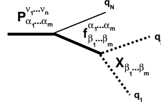
Fig. 2. Resonance decay into nucleon and two meson states
