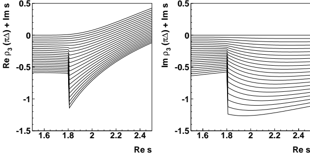
Fig. 6. The real (left-hand panel) and imaginary (right-hand panel) part of the \rho_3(s) as a function of Re s at fixed Im s_n = -20n MeV^2 , n = 1, 30 . For every n the curves are shifted down by the same step 20 MeV^2 .
