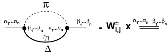
Fig. 4. Index definition in the \pi\Delta loop diagram
