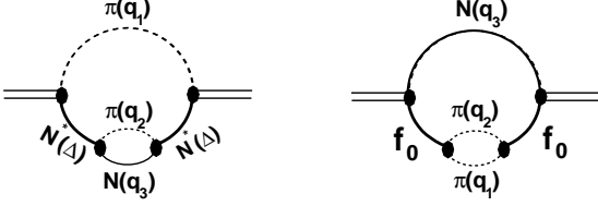
Fig. 3. \pi N^*(\pi\Delta) and f_0 N loop diagrams
