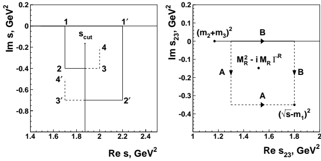
Fig. 5. The structure of threshold singularities in the s and s_{23} complex planes for the \pi\Delta channel.
